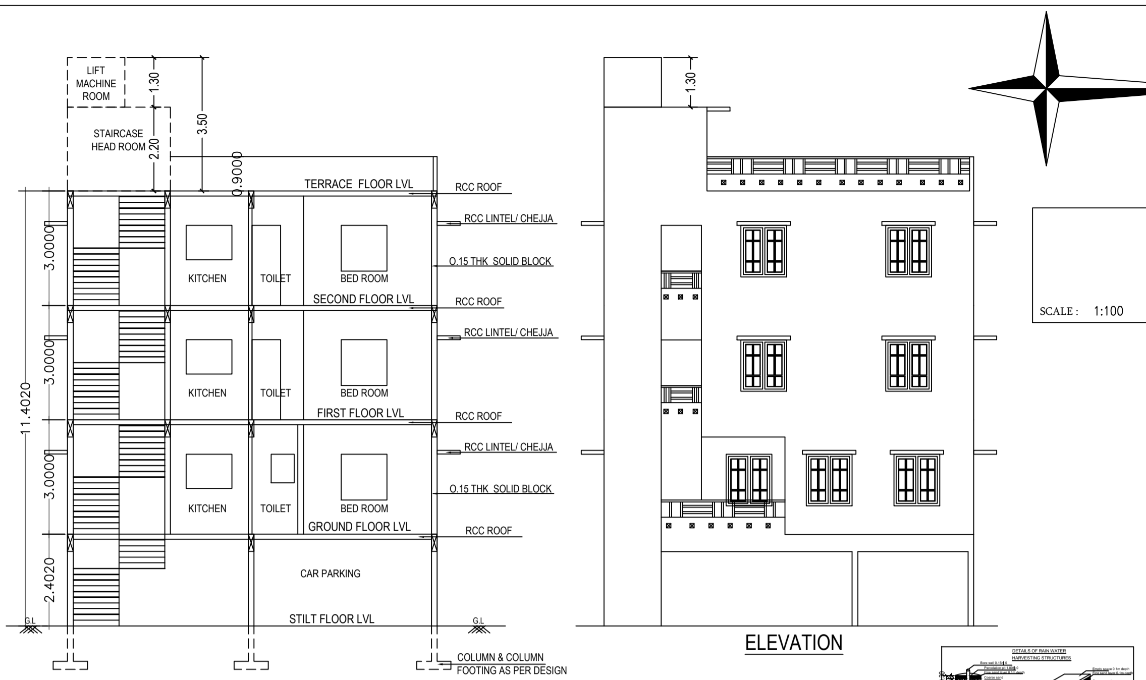
SECTION - AA
