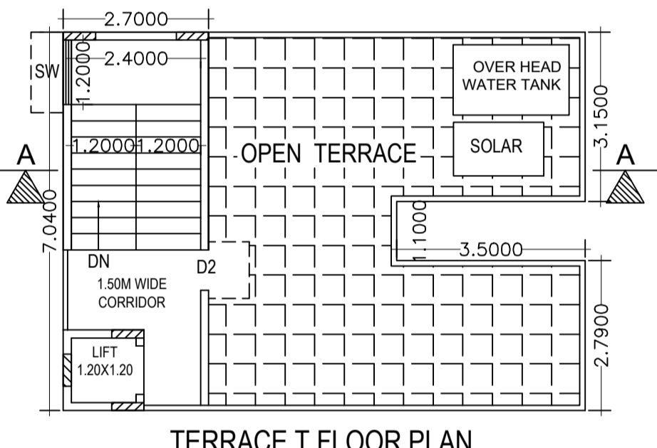
TERRACE T FLOOR PLAN
